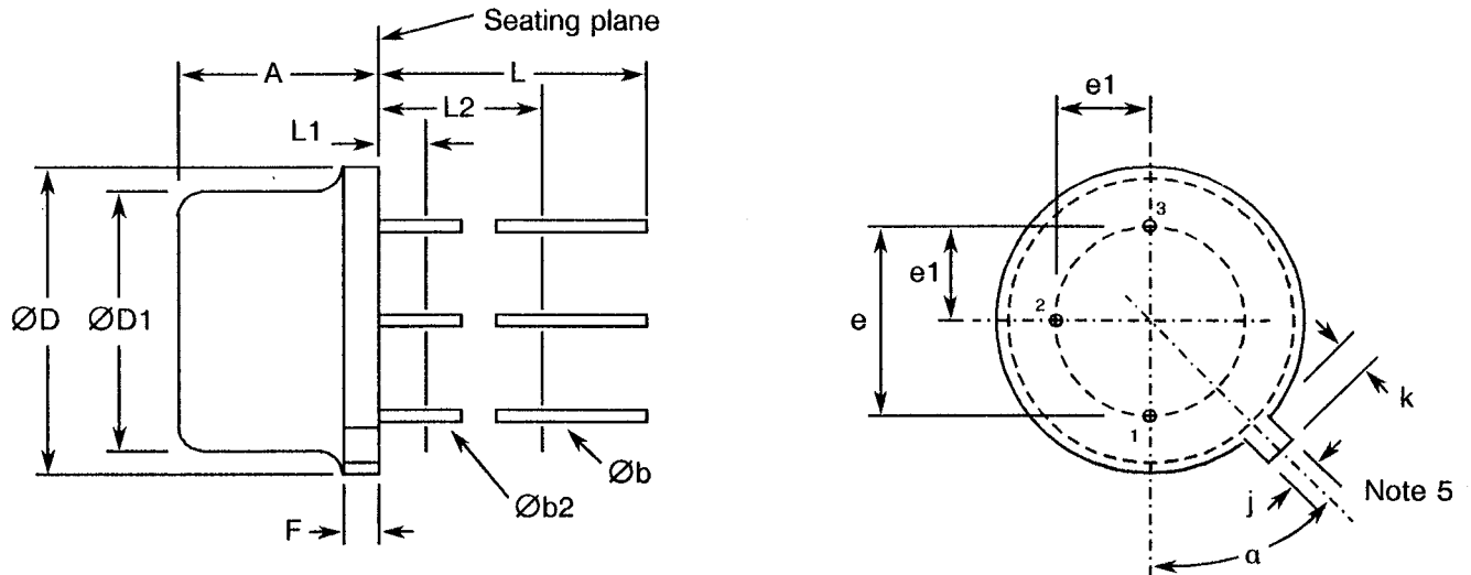
FIGURE 2 - PHYSICAL DIMENSIONS
