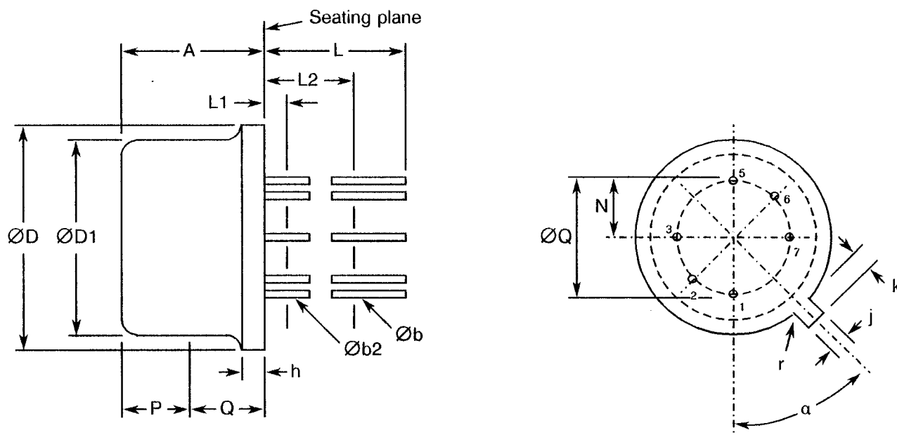
FIGURE 2(a) - VARIANT 01, TO-78 CAN
