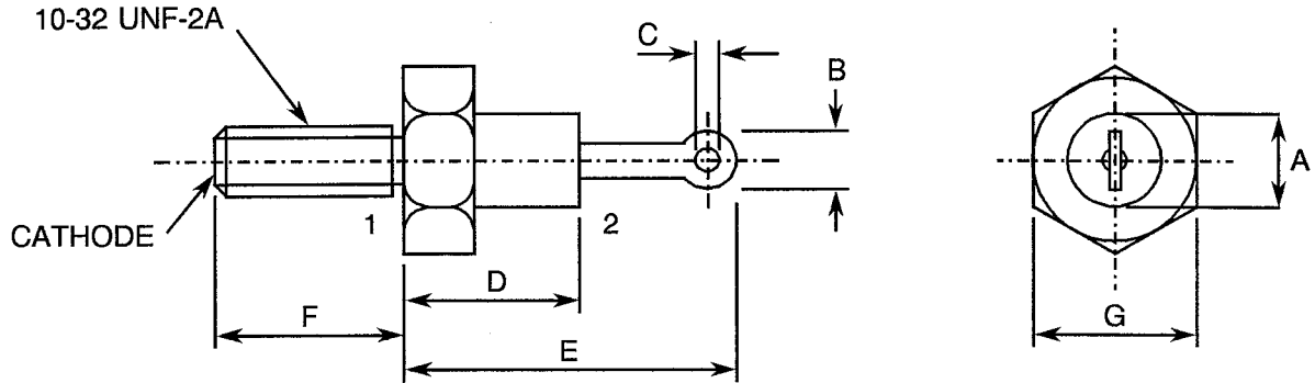
FIGURE 2 - PHYSICAL DIMENSIONS
