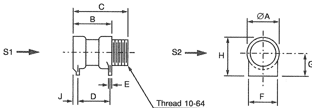
FIGURE 2(e) - VARIANT 05, STRIP LINE MOUNT
