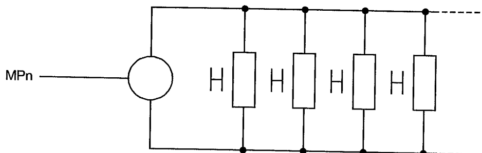
FIGURE 5 - CIRCUIT FOR BURN-IN AND OPERATING LIFE TESTS
