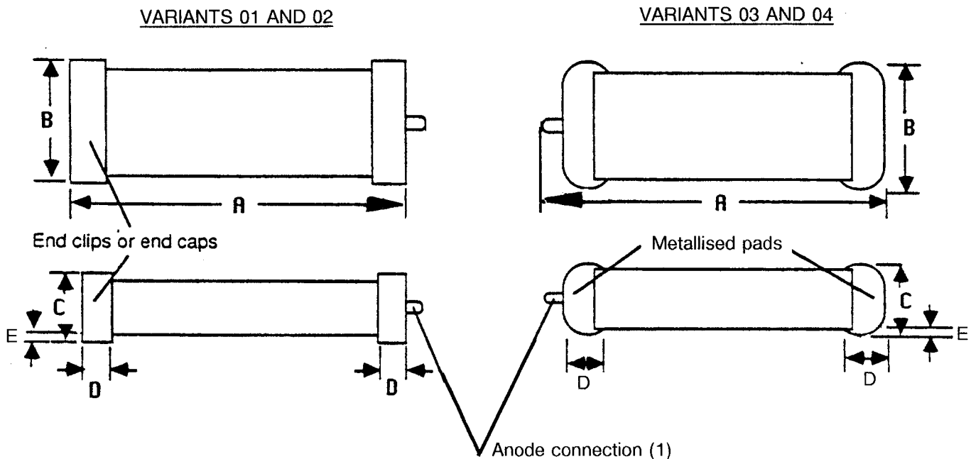
FIGURE 2 - PHYSICAL DIMENSIONS
