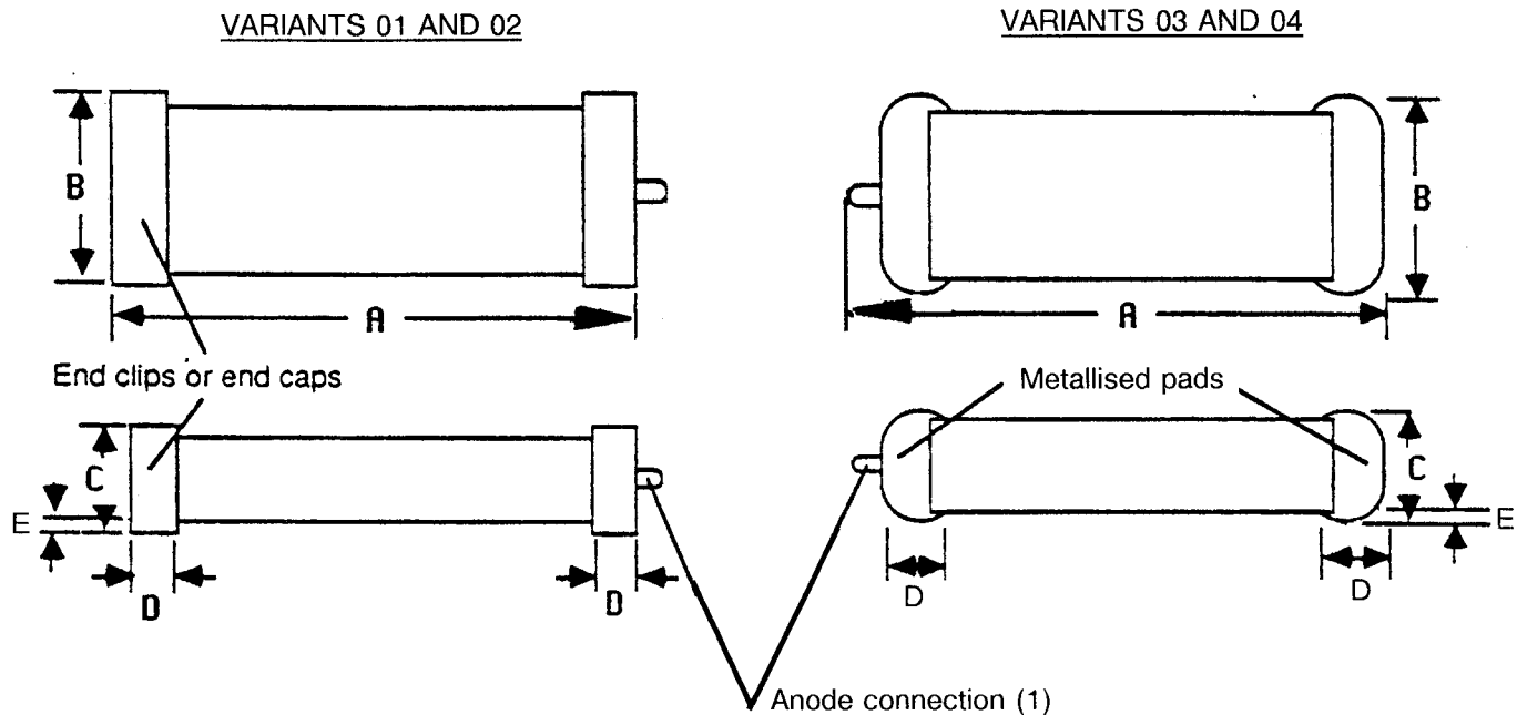
FIGURE 2 - PHYSICAL DIMENSIONS
