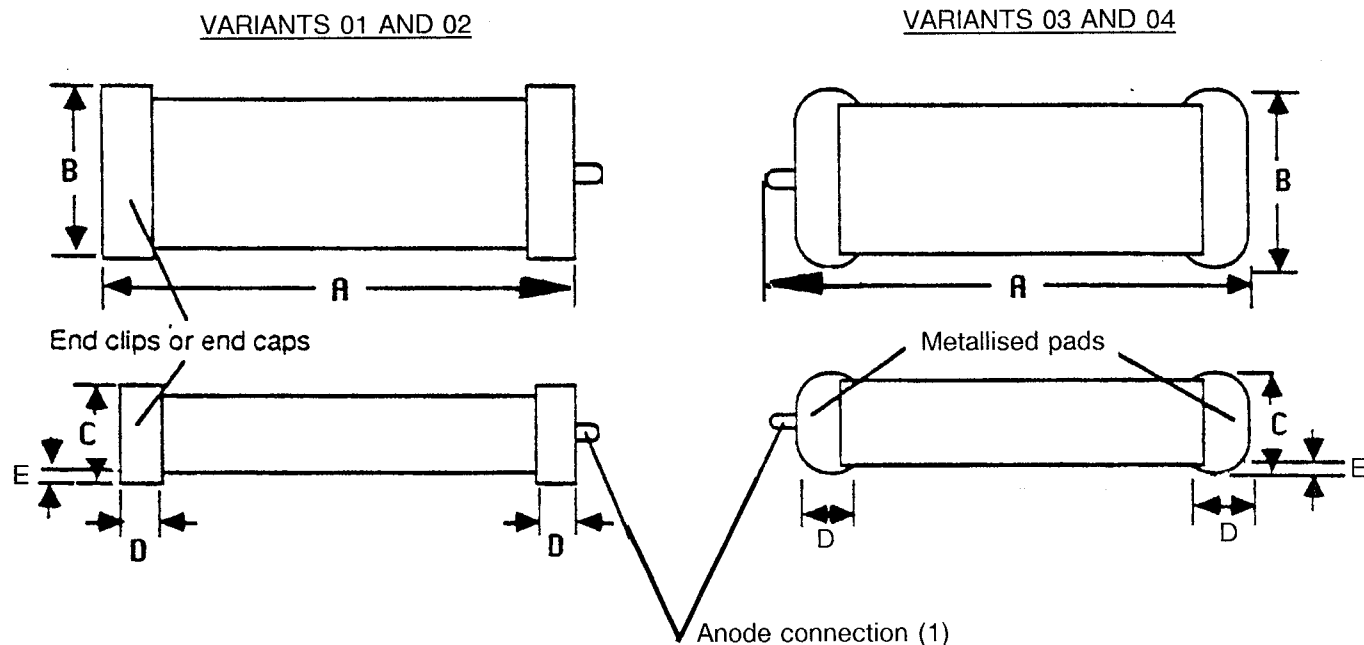
FIGURE 2 - PHYSICAL DIMENSIONS
