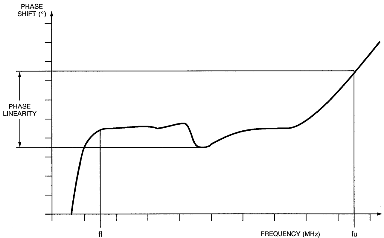
FIGURE IV - PHASE LINEARITY, TYPICAL PLOT
