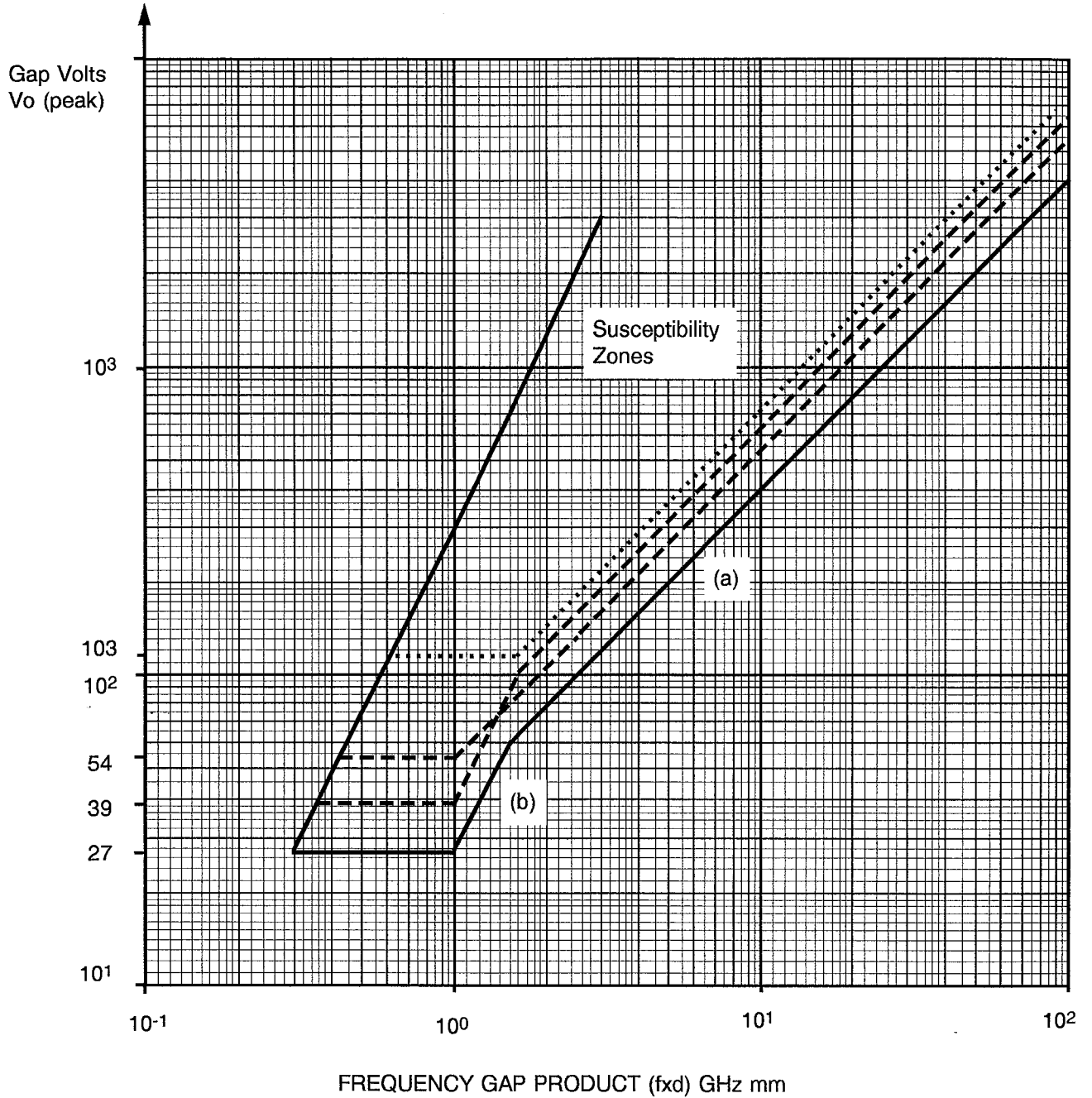
FIGURE VII - MULTIPACTION SUSCEPTIBILITY ZONES
