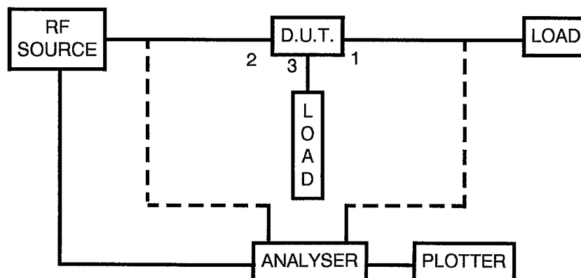
FIGURE III - CIRCULATOR ISOLATION TEST SET-UP
