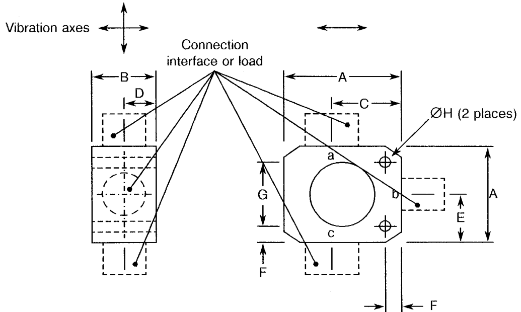
FIGURE 2(d) - 1/2" CONNECTORISED/DROP-IN
