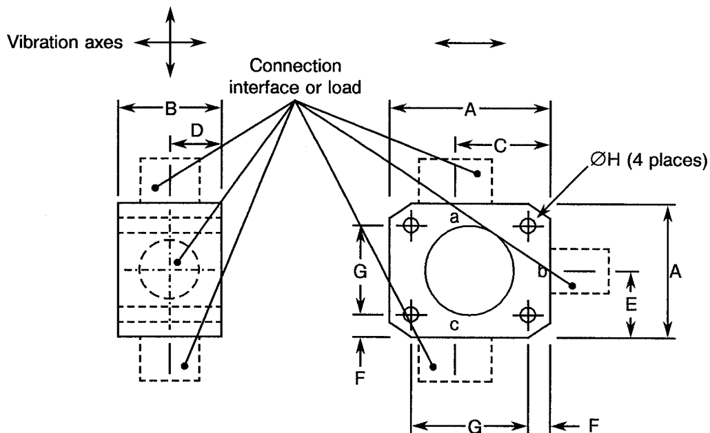
FIGURE 2(i) - 1" CONNECTORISED/DROP-IN
