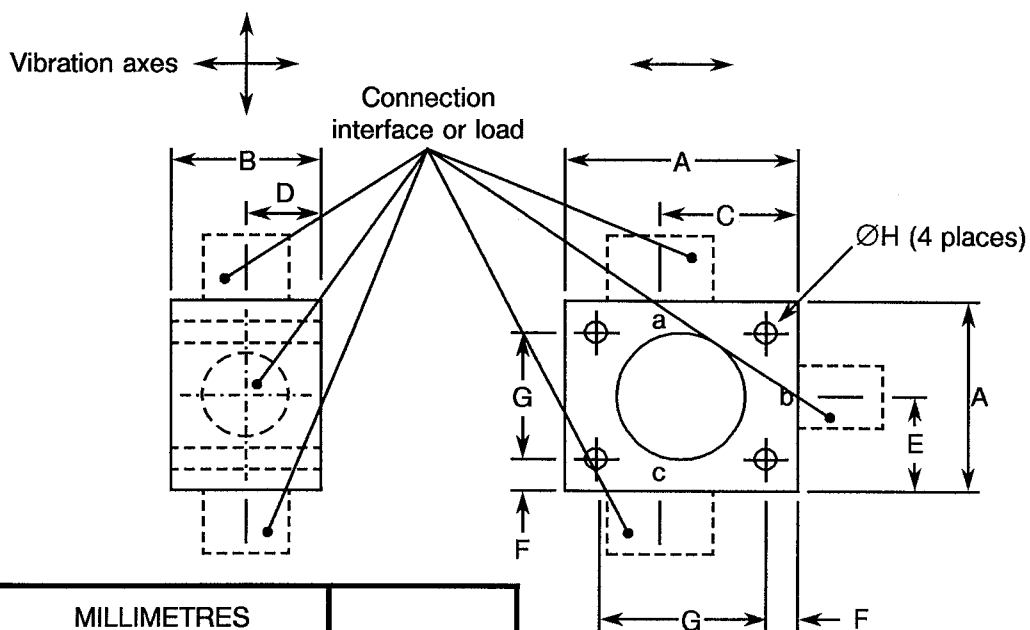
FIGURE 2(i) - 1 1/2" CONNECTORISED/DROP-IN
