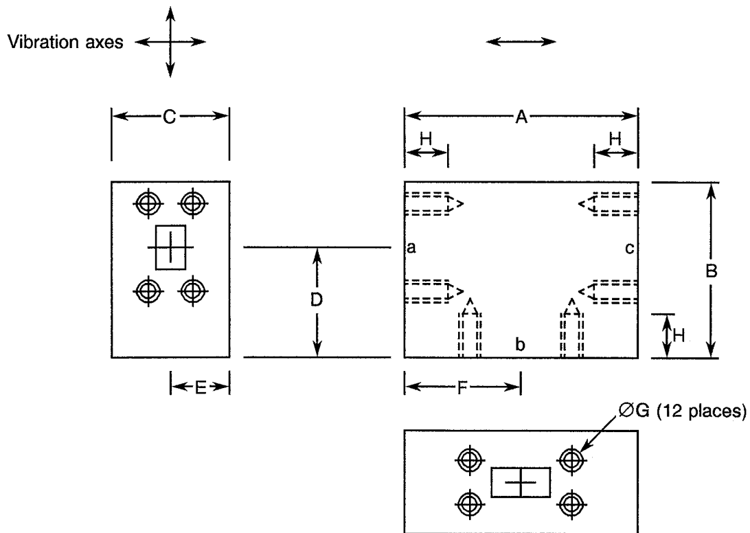
FIGURE 2 - PHYSICAL DIMENSIONS
