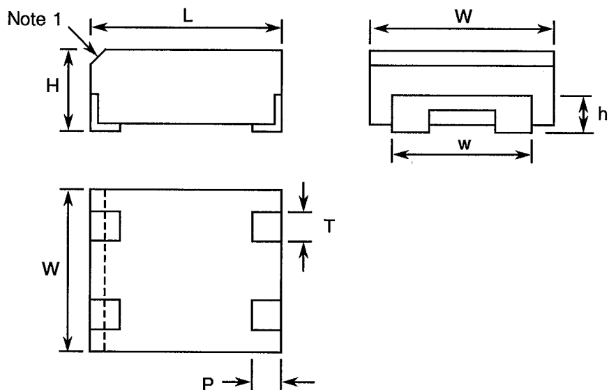
FIGURE 2 - PHYSICAL DIMENSIONS
