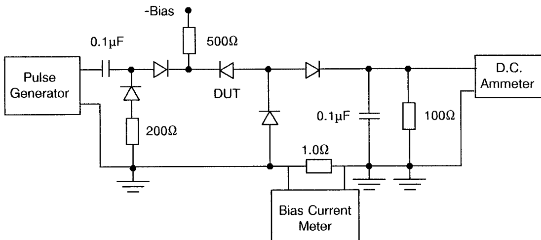
FIGURE 4(b) - MINORITY CARRIER LIFETIME
