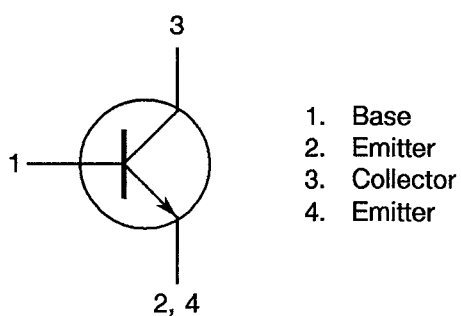
FIGURE 3 - FUNCTIONAL DIAGRAM
