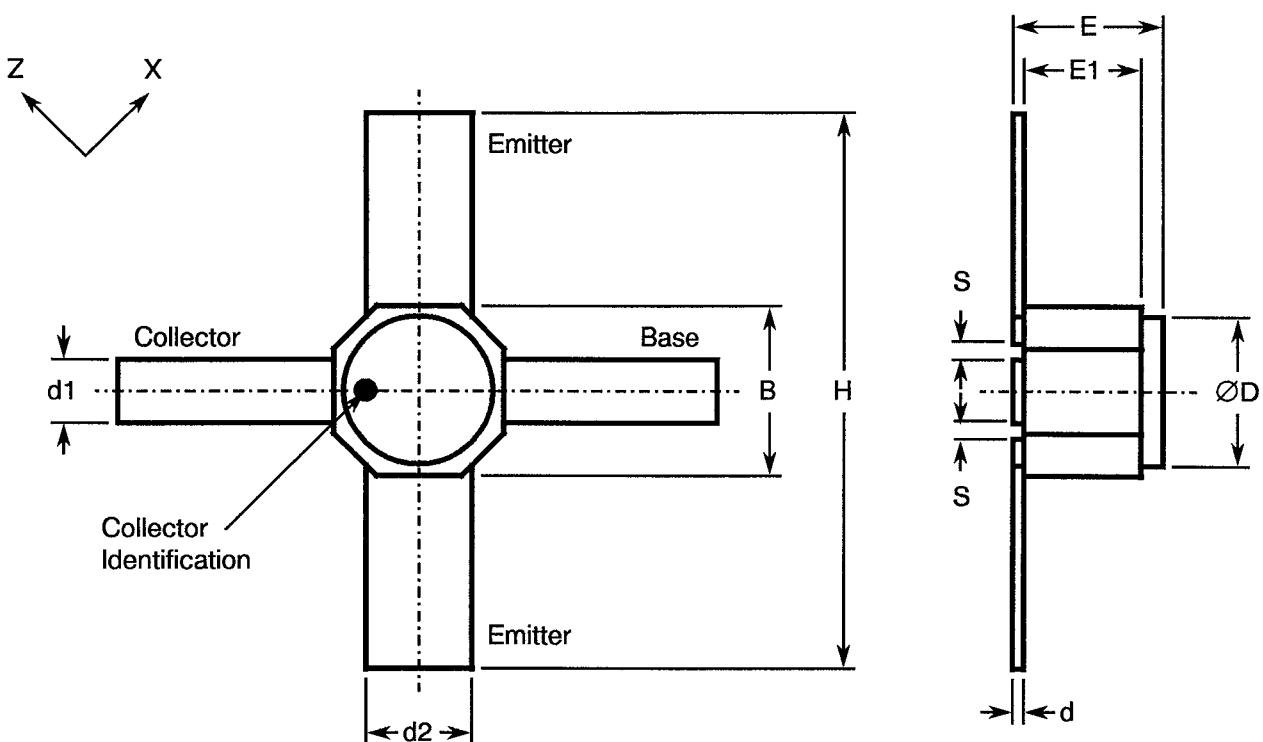
FIGURE 2 - PHYSICAL DIMENSIONS
