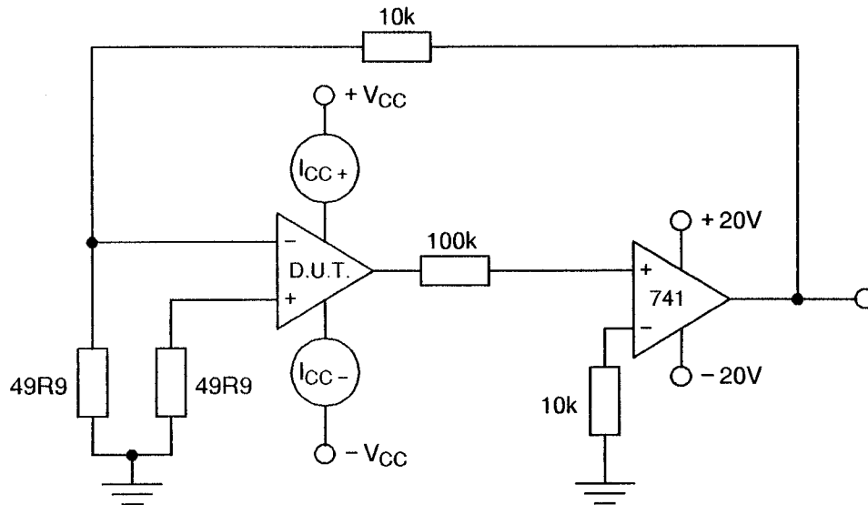
FIGURE 4(e) - SUPPLY CURRENT
