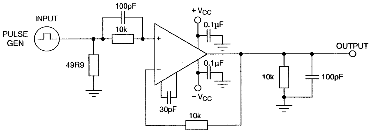
FIGURE 4(i) - DYNAMIC TEST MEASUREMENT CIRCUIT
