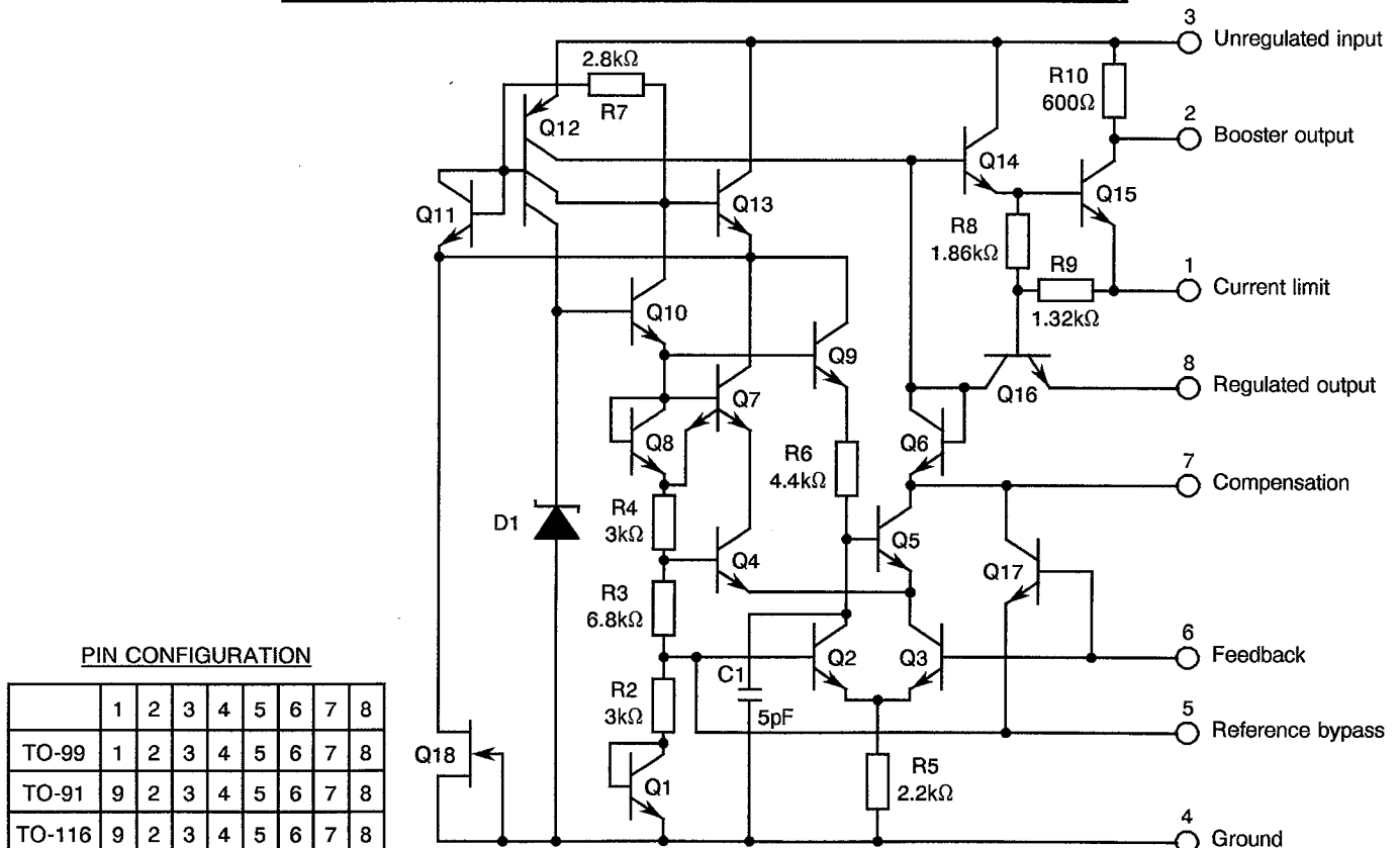
FIGURE 3(c) - CIRCUIT SCHEMATIC (FOR INFORMATION ONLY)
