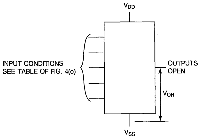
FIGURE 4(f) - HIGH LEVEL OUTPUT VOLTAGE
