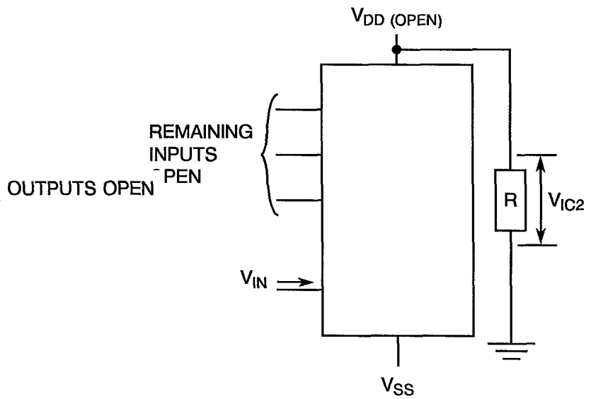
FIGURE 4(o) - INPUT CLAMP VOLTAGE ( V_{DD} )
