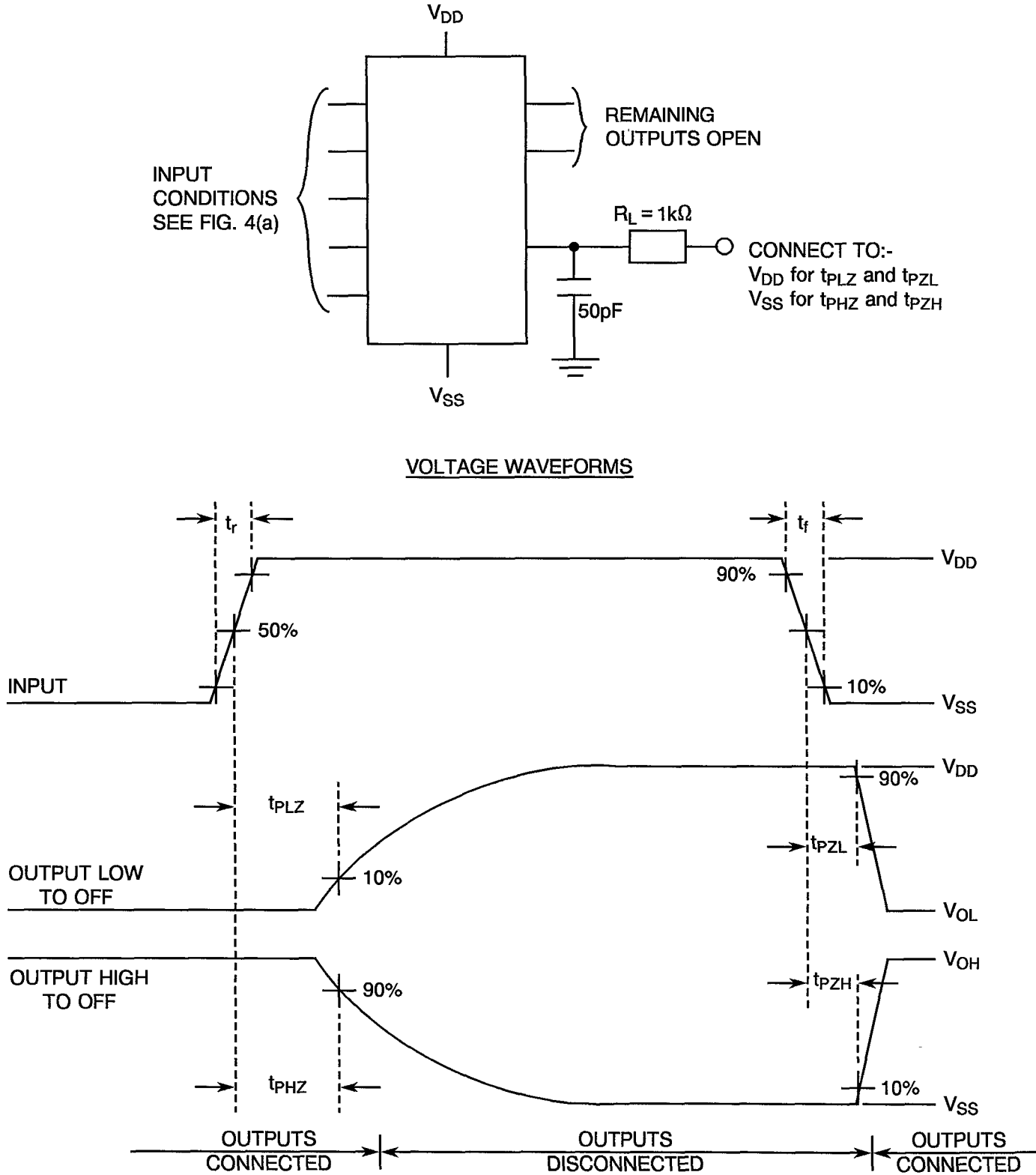
FIGURE 4(r) - PROPAGATION DELAY INPUT TO PHASE COMPARATOR II OUTPUT
