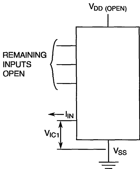
FIGURE 4(n) - INPUT CLAMP VOLTAGE ( V_{SS} )
