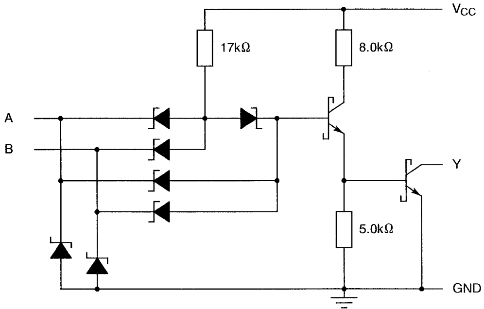
FIGURE 3(c) - CIRCUIT SCHEMATIC (EACH GATE)
