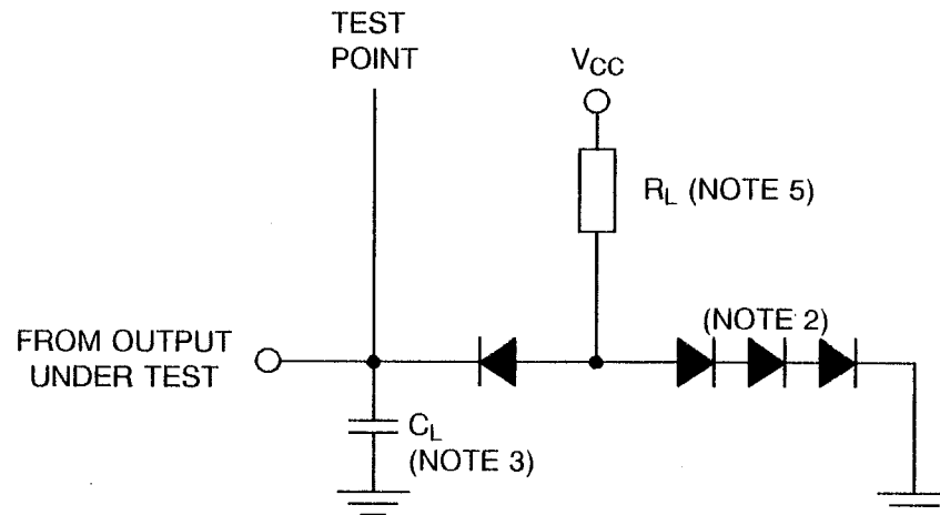
FIGURE 4(g) - DYNAMIC TEST AND SWITCHING WAVEFORMS
