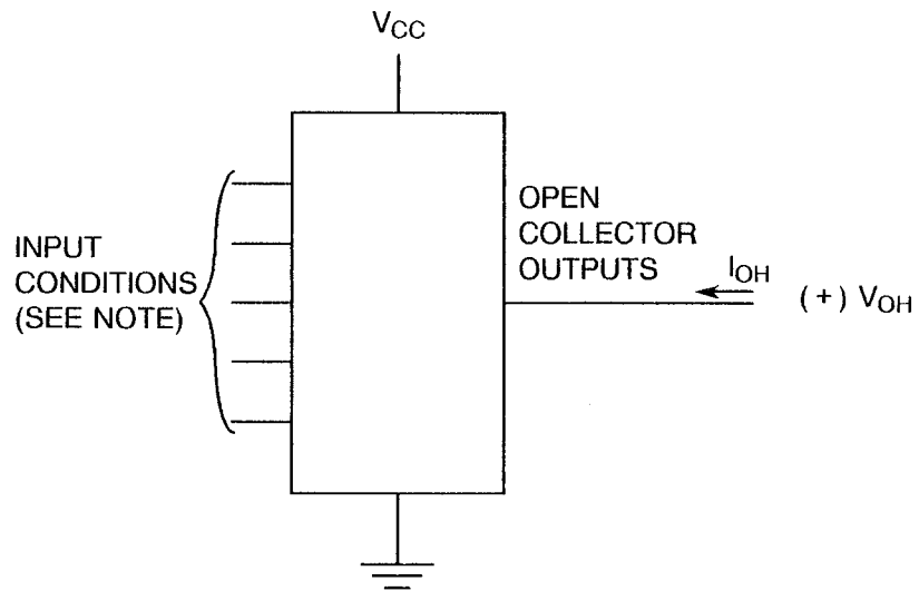
FIGURE 4(e) - HIGH LEVEL OUTPUT CURRENT
