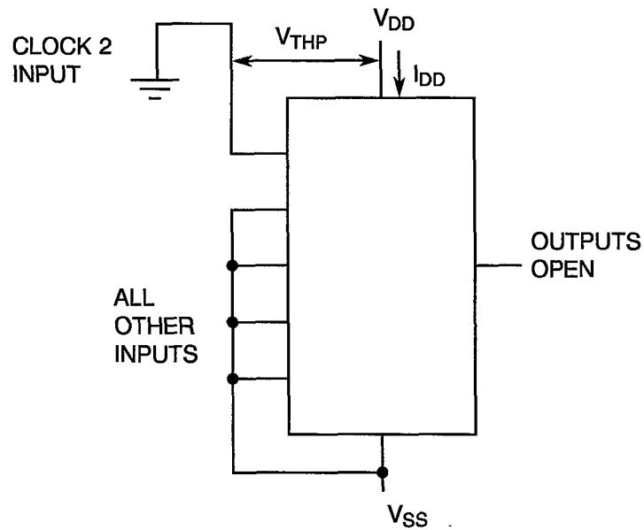
FIGURE 4(j) - THRESHOLD VOLTAGE P-CHANNEL
