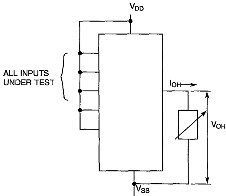
FIGURE 4(h) - HIGH LEVEL OUTPUT CURRENT
