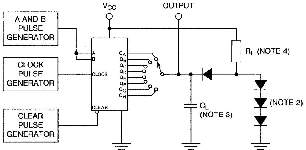
FIGURE 4(h) - DYNAMIC TEST AND SWITCHING WAVEFORMS
