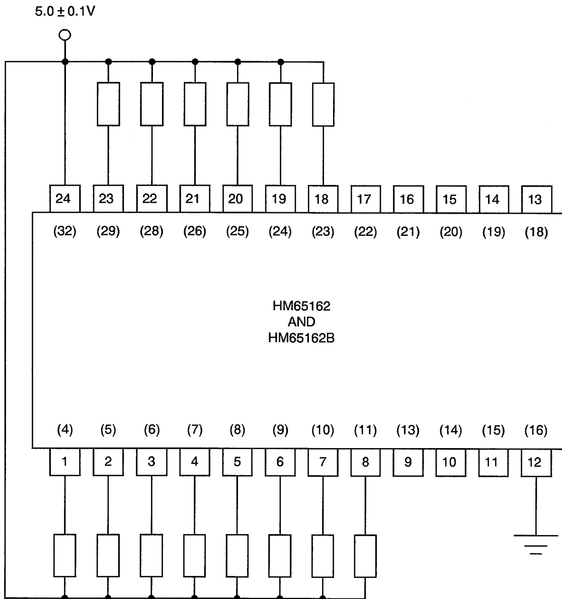
FIGURE 6 - BIAS CONDITIONS FOR IRRADIATION TESTING
