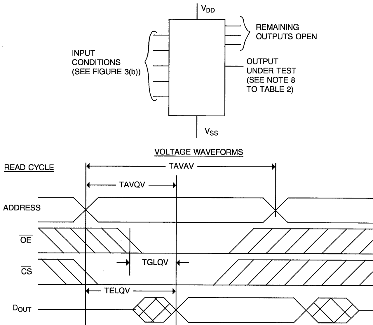
FIGURE 4(i) - PROPAGATION DELAY
