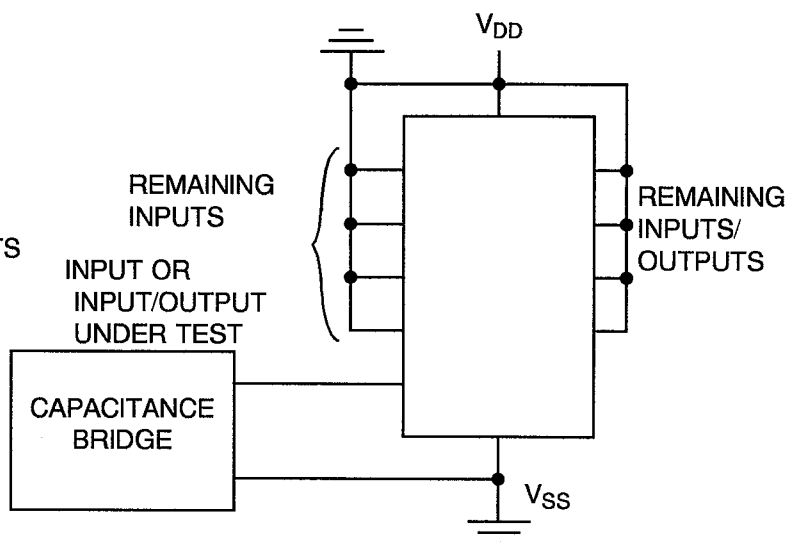
FIGURE 4(h) - INPUT OR INPUT/OUTPUT CAPACITANCE
