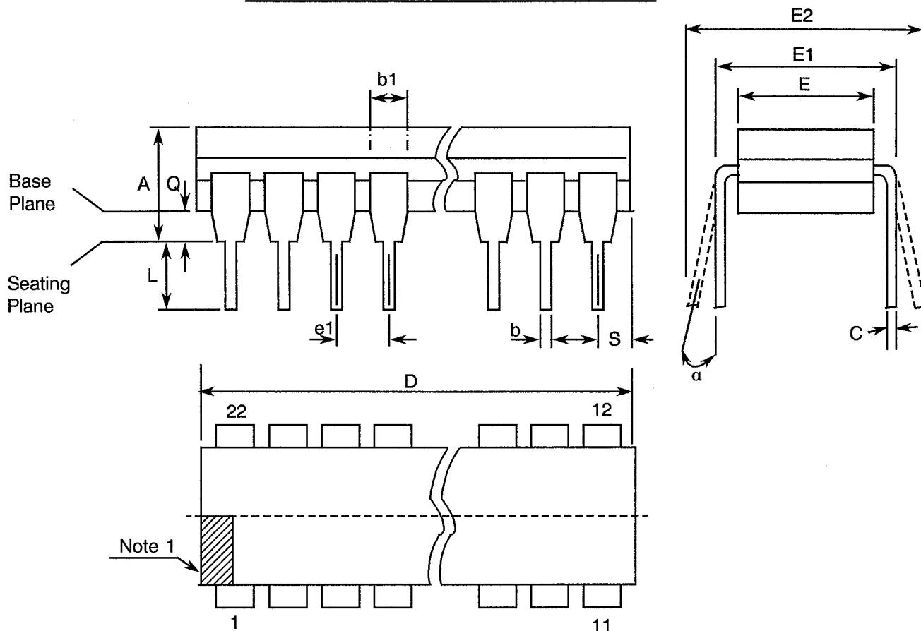
FIGURE 2(b) - DUAL-IN-LINE PACKAGE, 22 PIN
