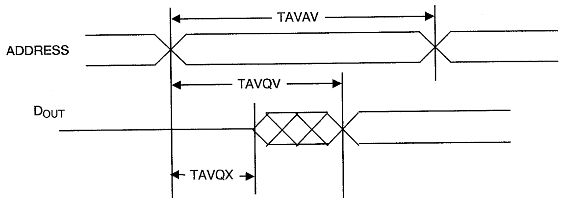
READ CYCLE 2
