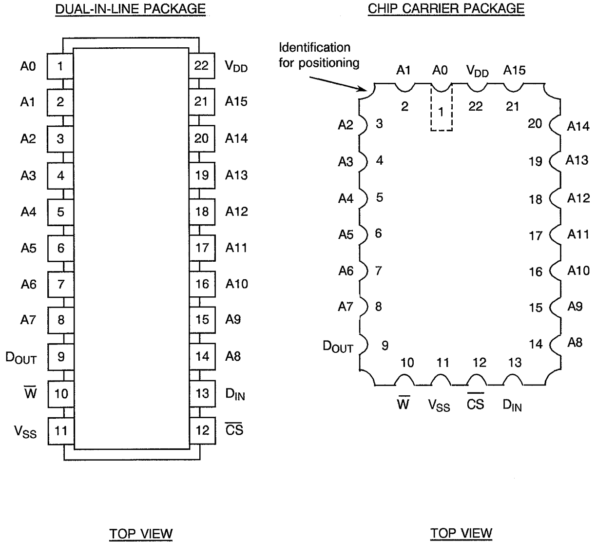
FIGURE 3(a) - PIN ASSIGNMENT
