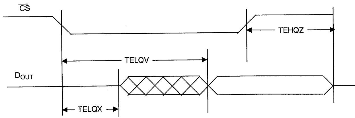
READ CYCLE 2
