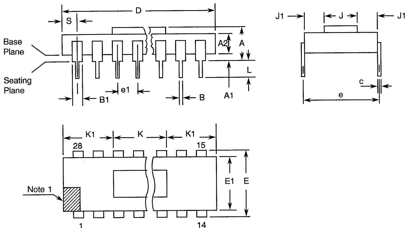
FIGURE 2(b) - DUAL-IN-LINE PACKAGE, 28 PIN
