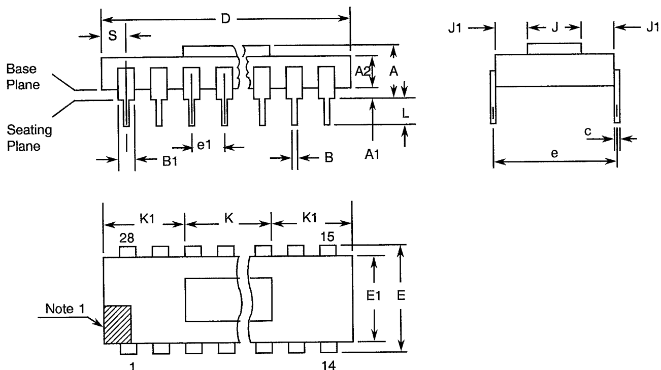
FIGURE 2(a) - DUAL-IN-LINE PACKAGE, 28 PIN
