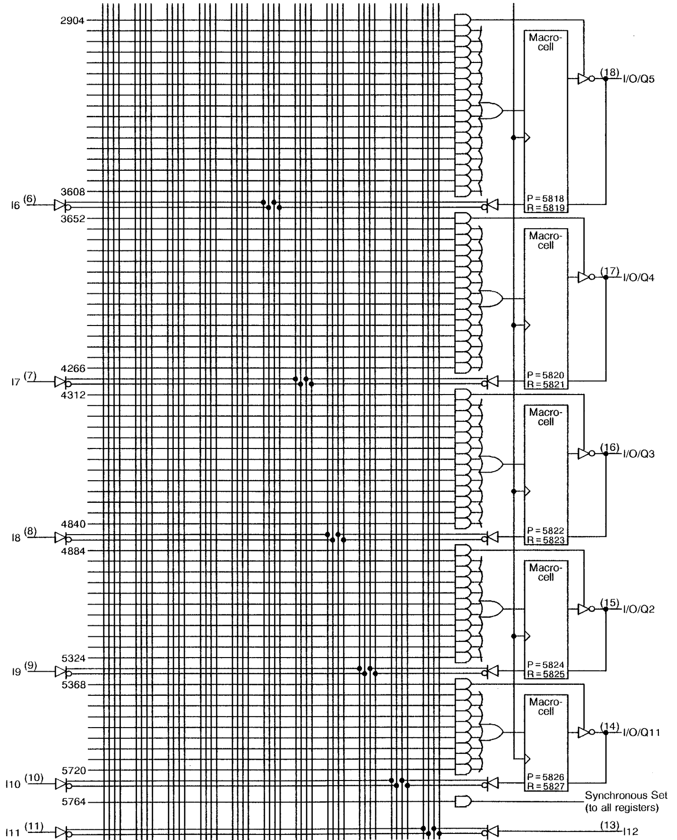
FIGURE 3(c) - PROGRAMMING MATRIX (CONTINUED)
