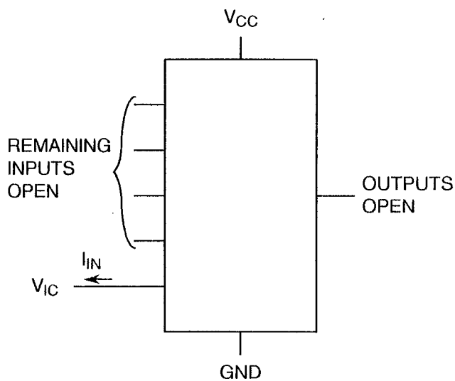
FIGURE 4(h) - INPUT CLAMP VOLTAGE
