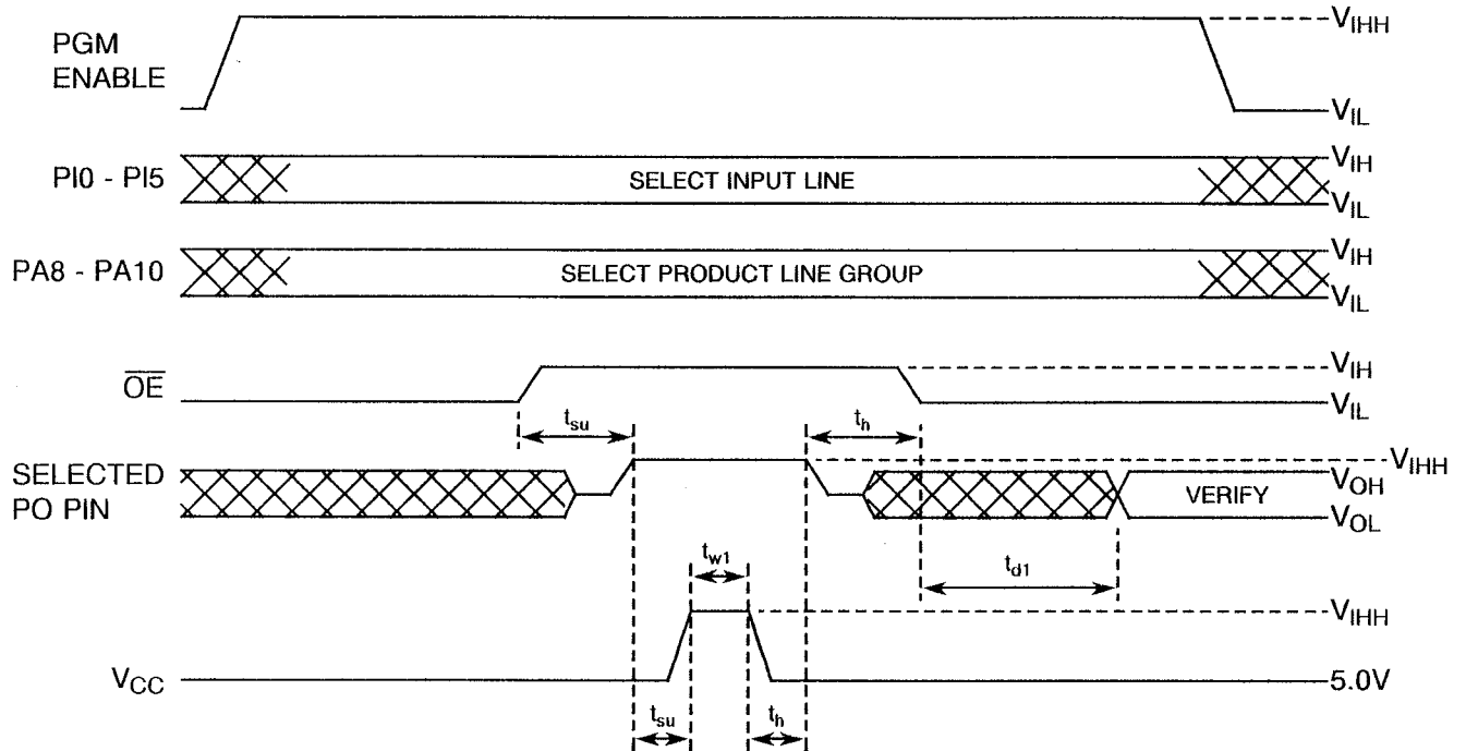
FIGURE II/1 - PROGRAMMING WAVEFORMS
