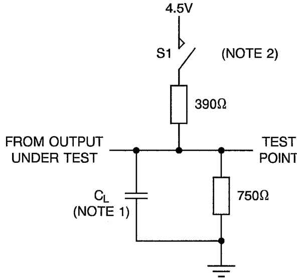
FIGURE 4(i) - PROPAGATION DELAY
