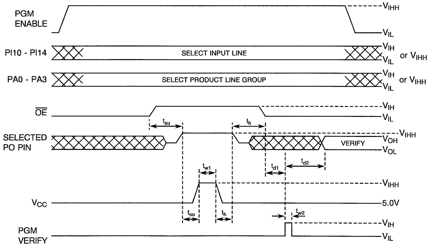
FIGURE II/2 - PROGRAMMING WAVEFORMS
