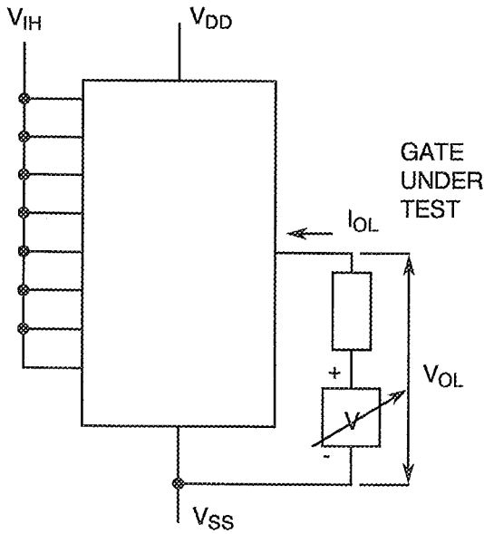
FIGURE 4(d) - OUTPUT VOLTAGE LOW LEVEL
