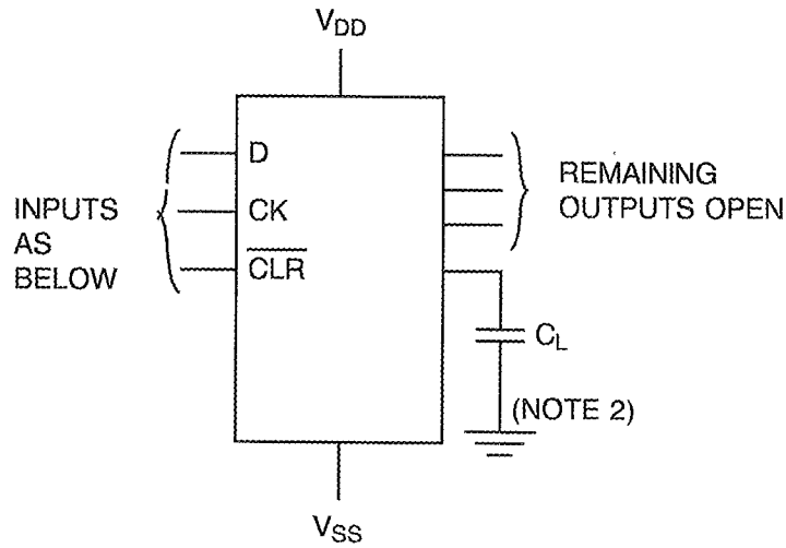
FIGURE 4(i) - PROPAGATION DELAY AND TRANSITION TIME
