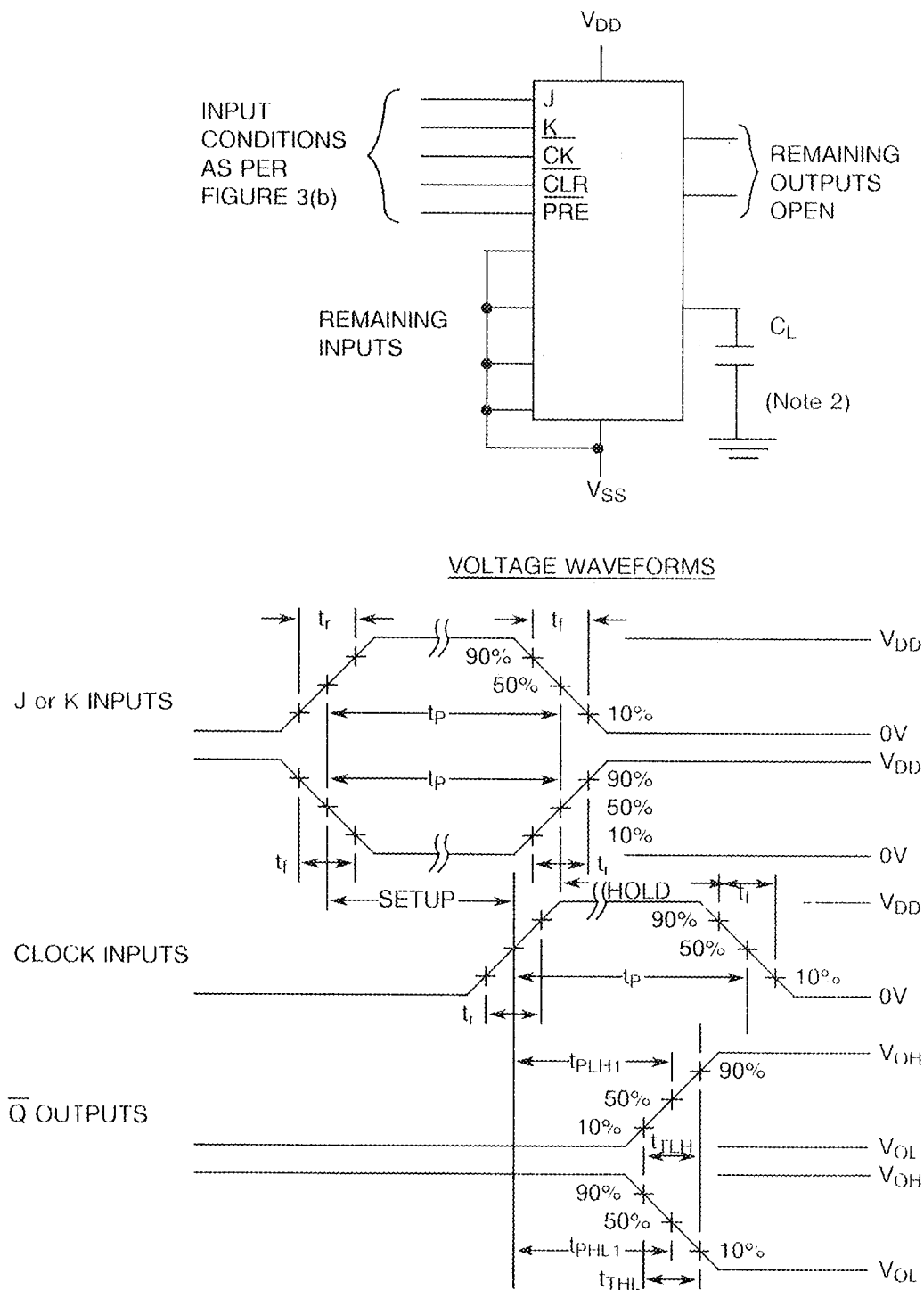
FIGURE 4 (i) - PROPAGATION DELAY AND TRANSITION TIME
