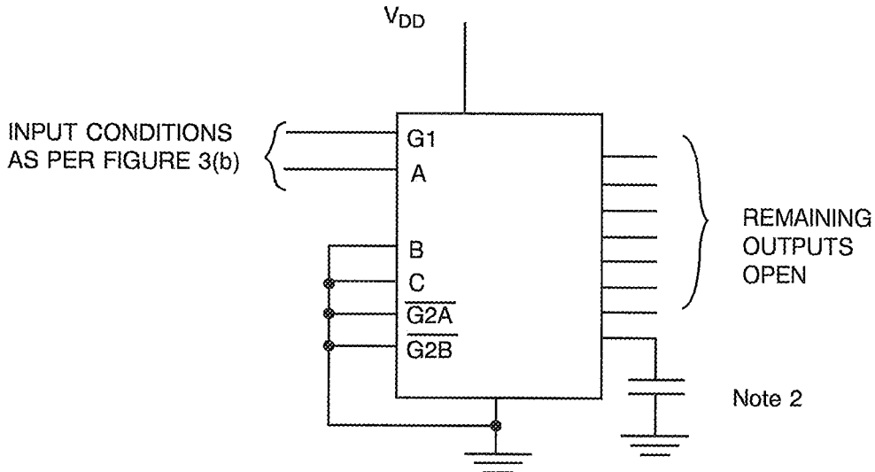
FIGURE 4(j) - PROPAGATION DELAY AND TRANSITION TIME
