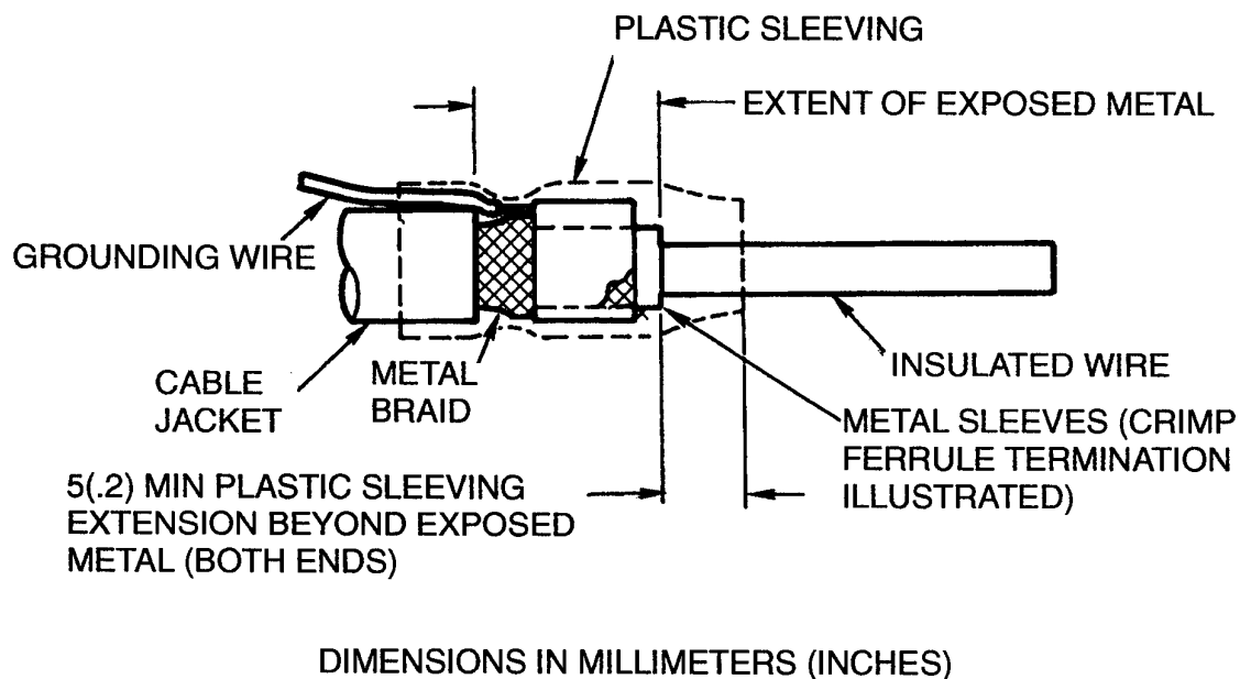
Figure 9-13. Illustration of Shrink Sleeve Installation (Typical)
