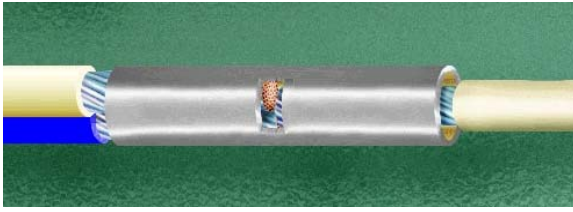
Figure 19-29. Butt Splice Prior to Crimp Figure 19-30. Properly Crimped Butt Splice
