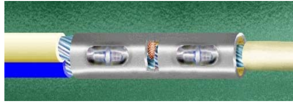
Figure 19-29. Butt Splice Prior to Crimp Figure 19-30. Properly Crimped Butt Splice
