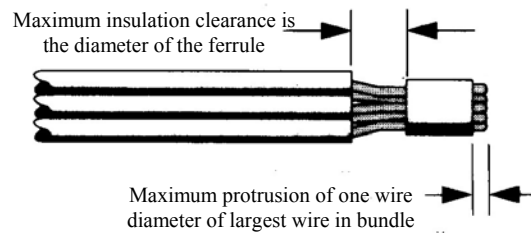
Figure 19-18. Solder Ferrule
