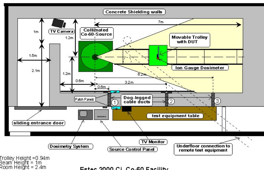
Estec 2000 Ci Co-60 Facility
