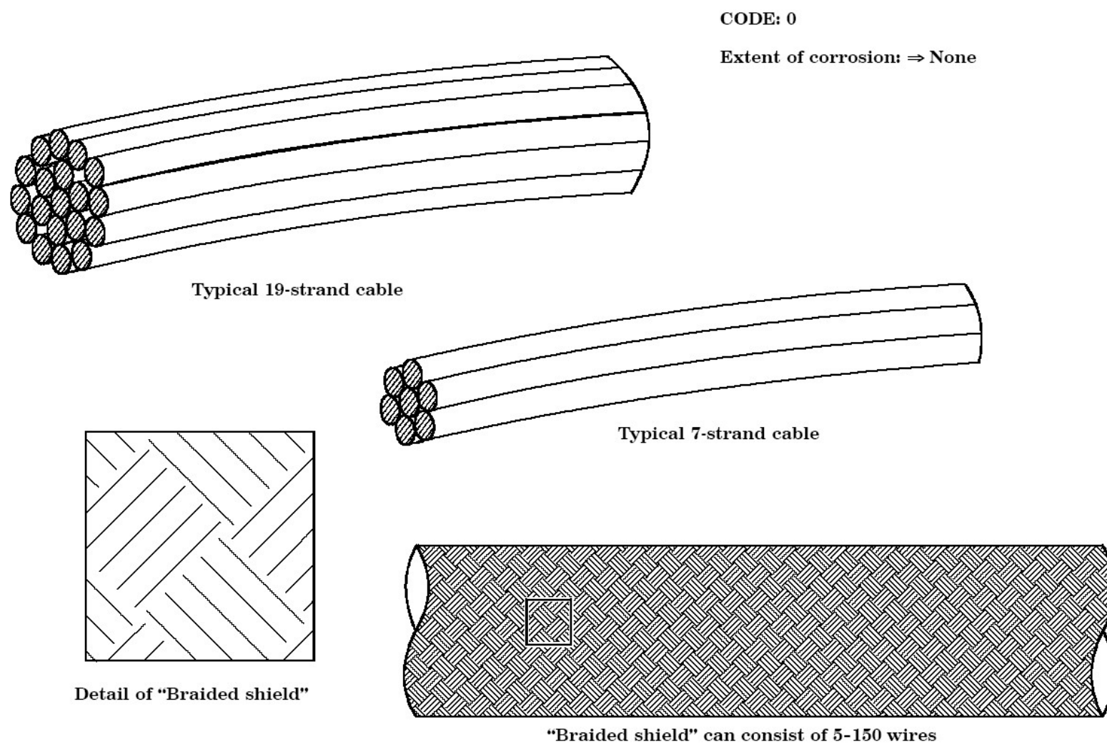
Figure C-1: Extent of Corrosion (per 20 cm length/test sample): Code 0
