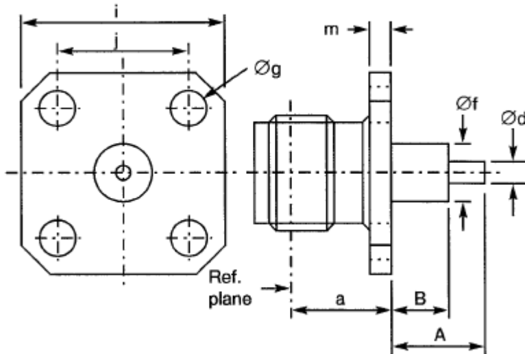
VARIANT 03 – SQUARE FLANGE RECEPTACLE
