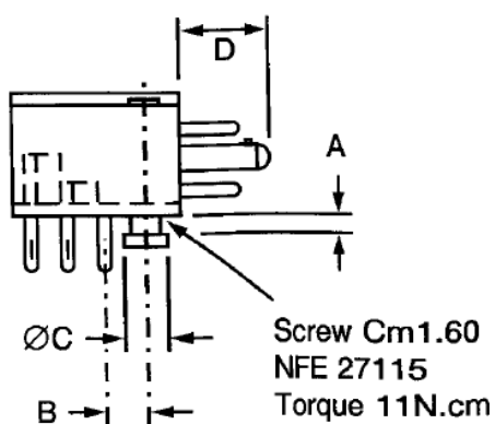
FIGURE 2(b) – GUIDING AND LOCKING DEVICES
