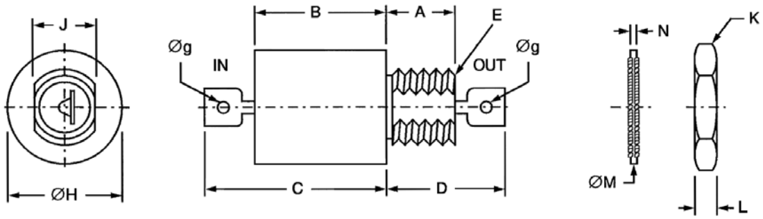
FIGURE 2 – PHYSICAL DIMENSIONS
