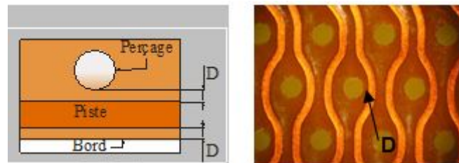
Figure 10-88: Misregistration of hole in coverlay to the conductor
