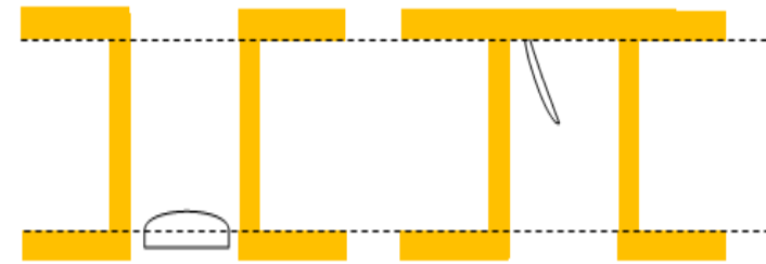
Figure 10-29: Examples of unacceptable voids
