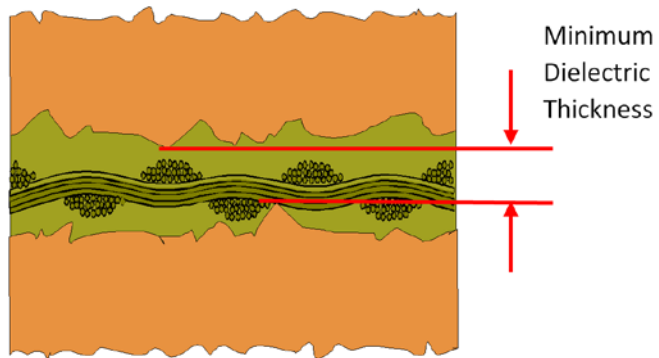
Figure 10-12: Projected-peak-to-peak insulation
