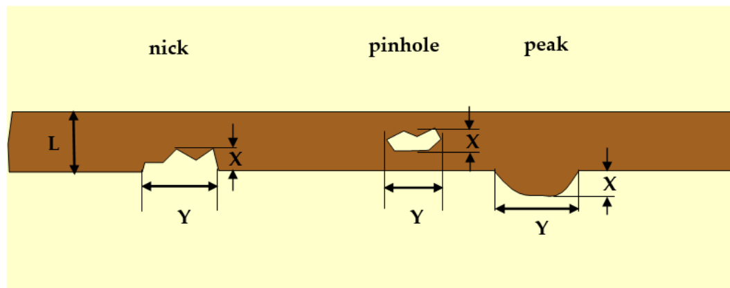
Figure 10-67: Conductor width
