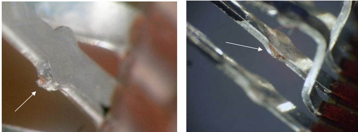
Figure 10-92: Bare copper on fingers
