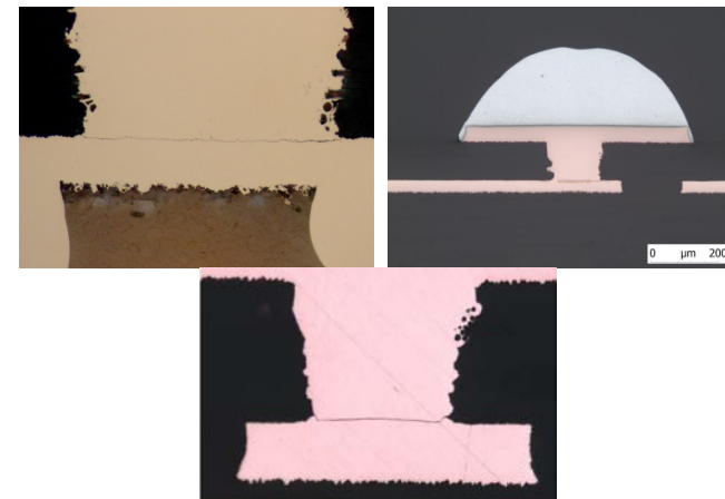
Figure 10-18: ICD on capture pad (pictures are unetched)
