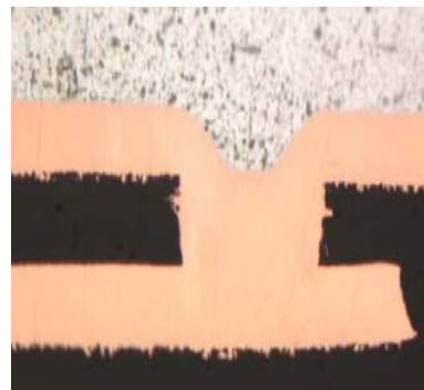
Figure 10-17: Dimple in microvia
