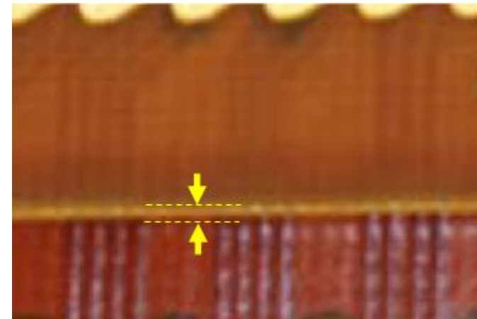
Figure 10-81: Example of adhesive fillet recession into rigid section as observed in visual inspection
