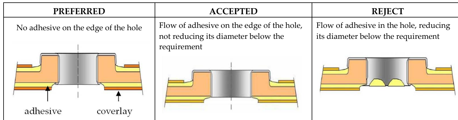
Figure 10-98: Adhesive in plated holes
