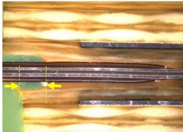
Figure 10-66: Example of adhesive filet recession into rigid section as observed in microsection
