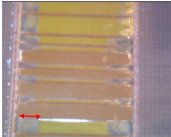
Figure 10-80: Example of resin squeeze out
