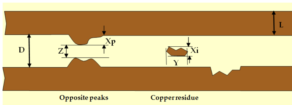
Figure 10-68: Conductor spacing
