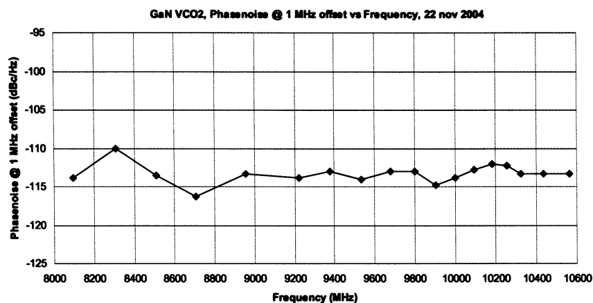
Figure 9 measured phase noise of the VCO versus carrier frequency
