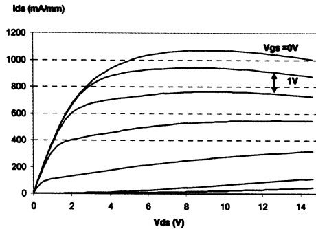
Figure 19. DC (I-V) characteristics to a 2 \times 50 \mu\text{m} \times 0.17 \mu\text{m} AlGaN/GaN HEMT (gate to drain spacing of 2.5 \mu\text{m} )
