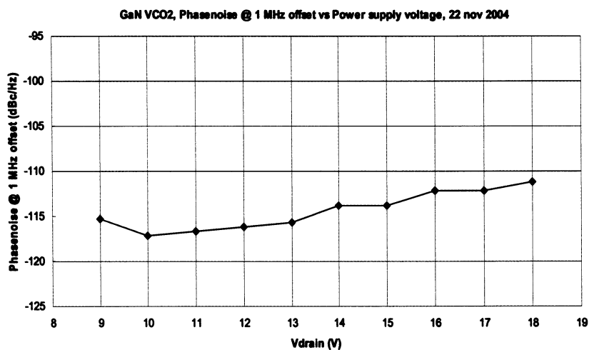
Figure 10 measured phase noise of the VCO versus Vdrain
