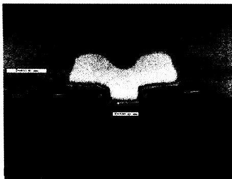
Figure 11. 0.15µm mushroom gate
