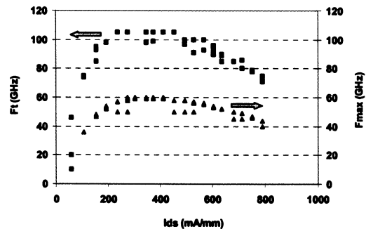
Figure 20. Unity current gain cut-off frequency ( f_T ) and maximum frequency of oscillation ( f_{\text{max}} ) against drain current for 0.17 \times 100 \mu\text{m}^2 V_{\text{ds}} = 10\text{V} and I_{\text{ds}} = 235\text{mA/mm} .
