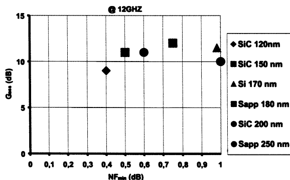
Figure 28. State of the art of G_{ass} versus NF_{min} at 12GHz for different GaN devices. The blue triangle corresponded to the estimated G_{ass} / NF_{min} of GaN HEMT on Silicon.
