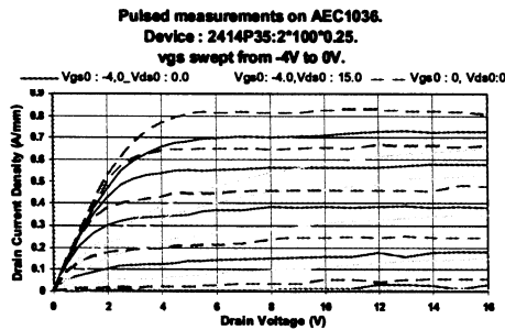
Figure 23. AEC1026 I_{ds} - V_{ds} curves for gate pulse of 600ns, drain pulse : 550ns every 10 \mu s
