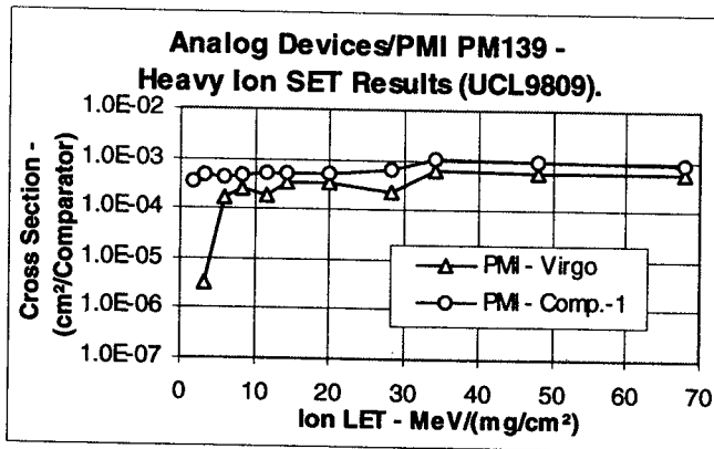
Figure 19. Heavy ion SET results – Analog D./PMI PM139.
