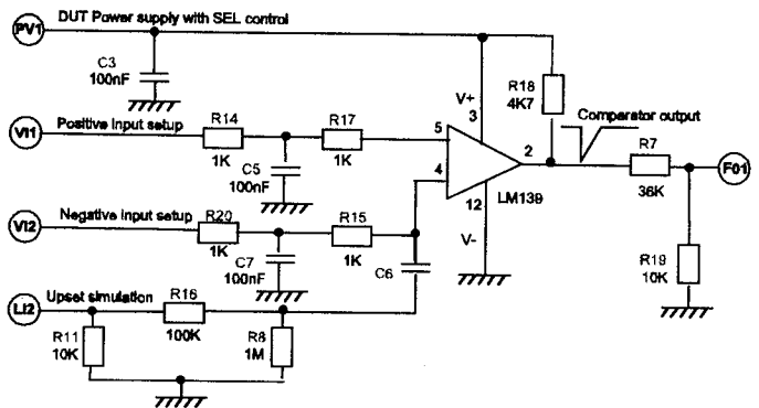
Figure 18. LM/PM139 Comparator Test schematics/set-up
